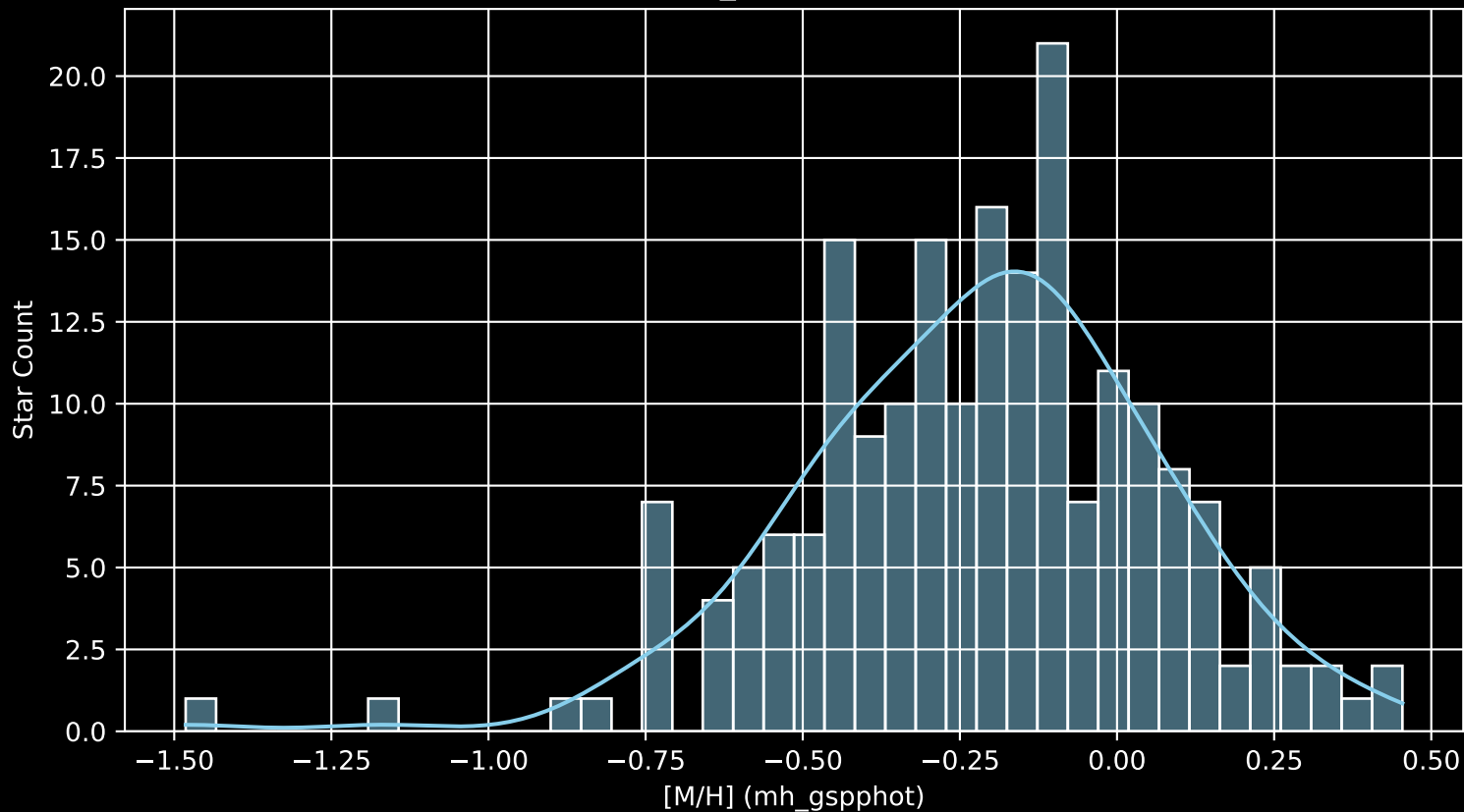
APOGEE DR17 Field: [067+46_MGA [M/H] (mh_gspphot) (n= 199)
