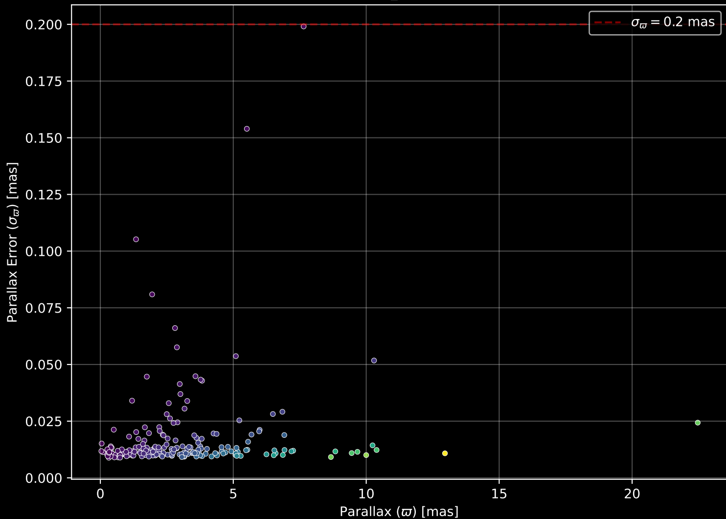
APOGEE DR17 Field: [067+46_MGA] Parallax Quality (n= 202)
