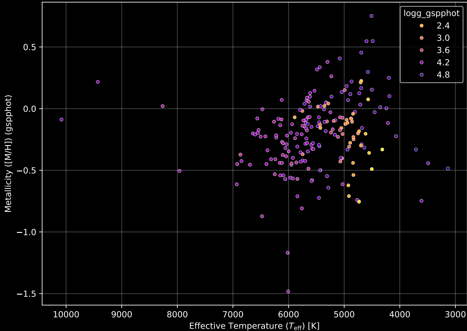
APOGEE DR17 Field: [067+46_MGA] Stellar Population Parameters (n= 202)
