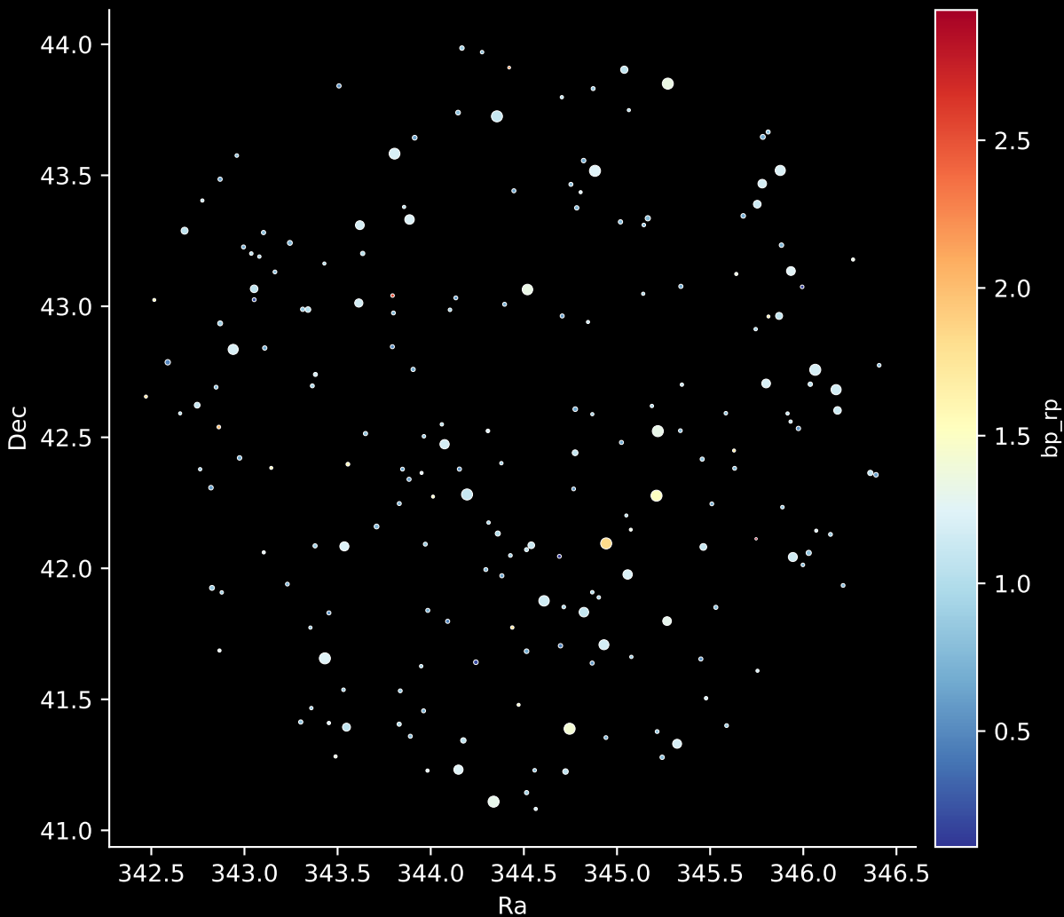
APOGEE DR17 Field: [067+46_MGA] Stars: 202
