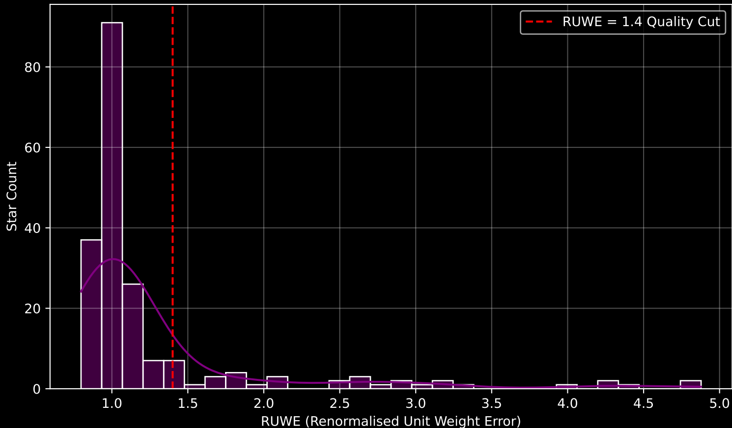
GAPOGEE DR17 Field [067+46_MGA] RUWE Distribution (n= 198)
