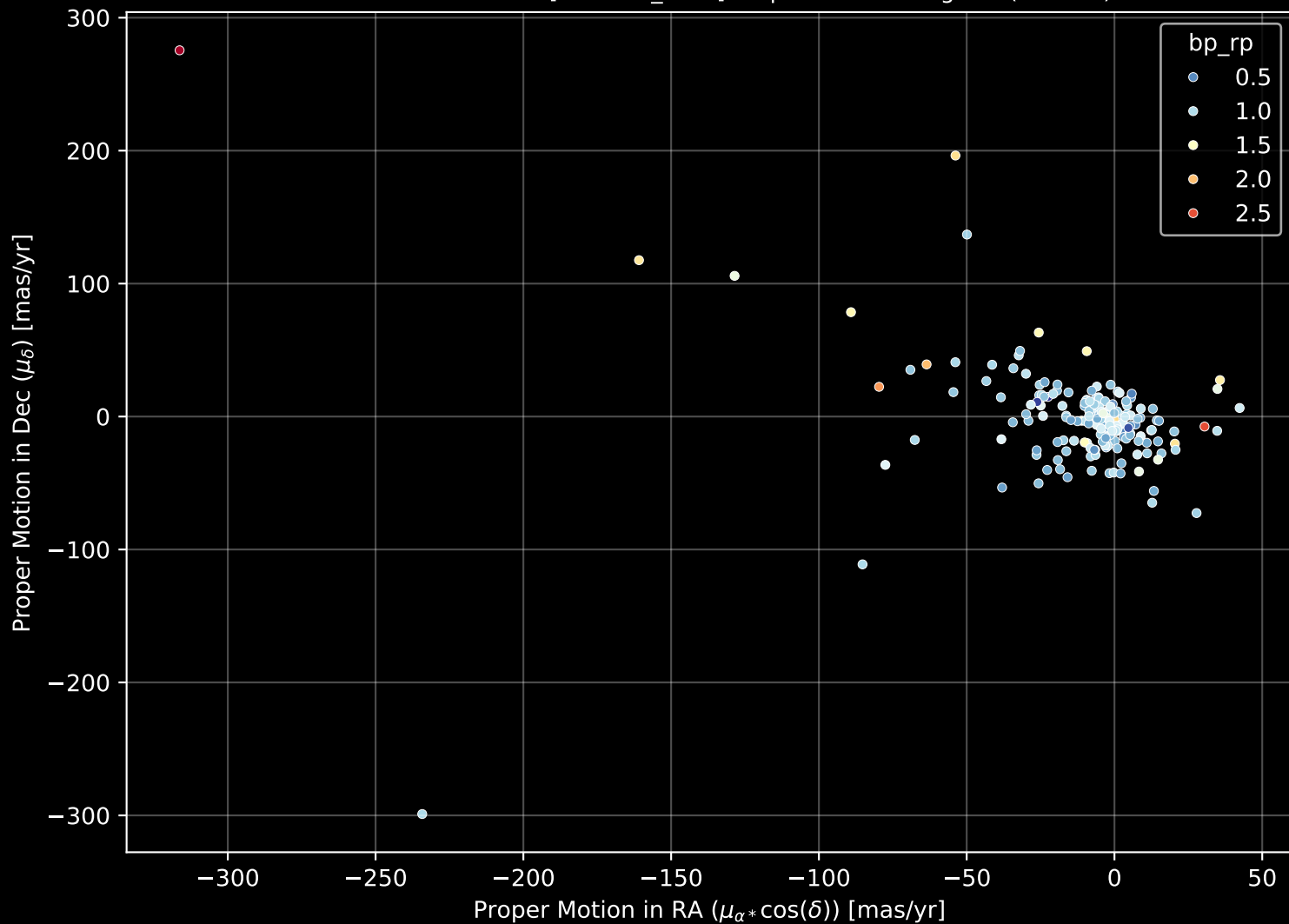
APOGEE DR17 Field: [067+46_MGA] Proper Motion Diagram (n= 202)
