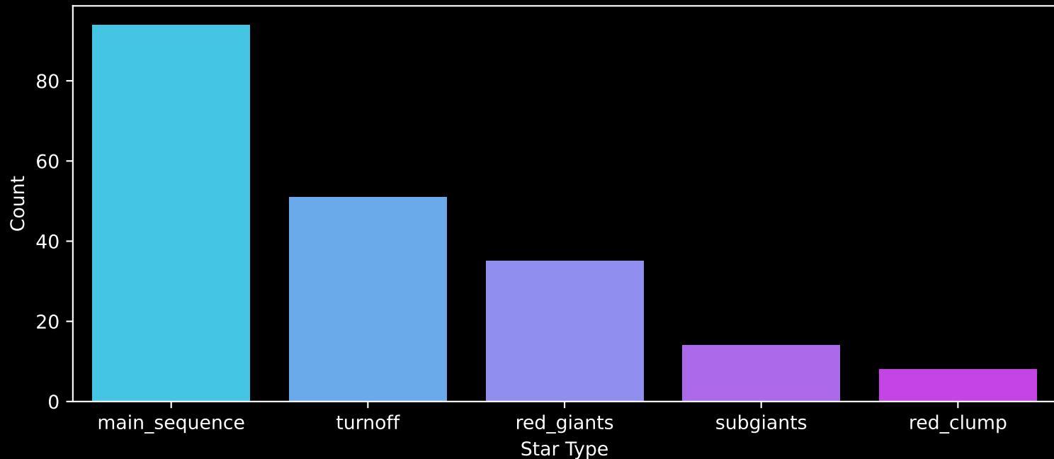
APOGEE DR17 Field: [067+46_MGA] Count plot of Star Type
