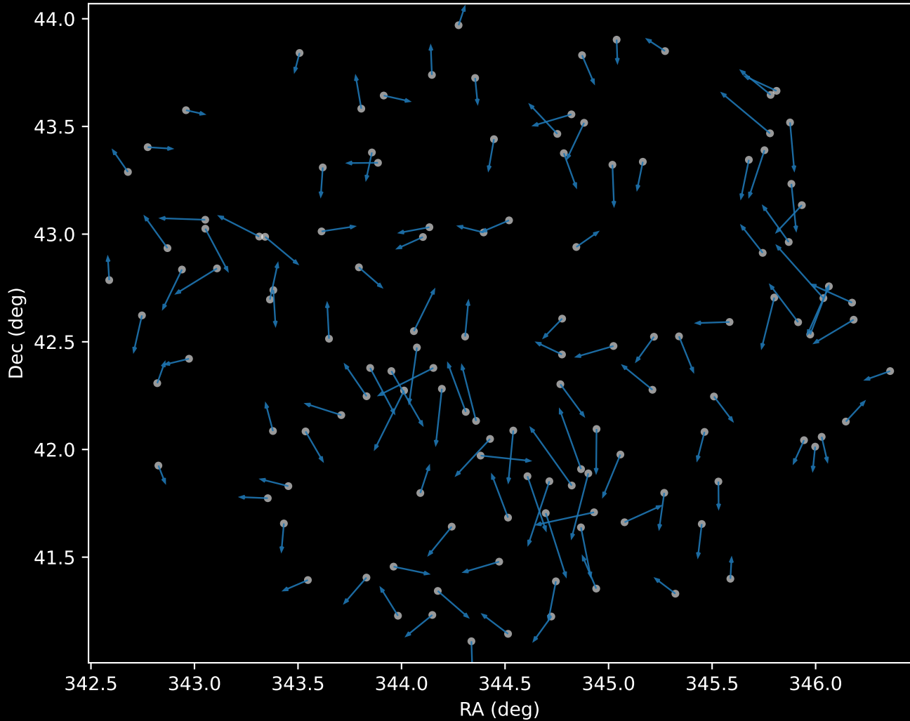
APOGEE DR17 Cluster 0 Proper Motion Vectors (n=127)
